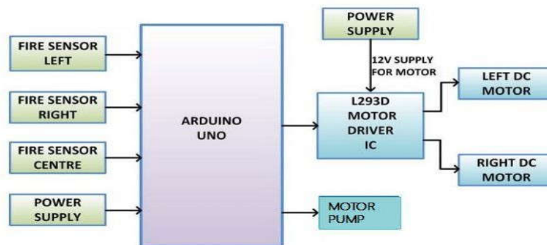
Fig-3: Block Diagram of Fire Fighting Robot
