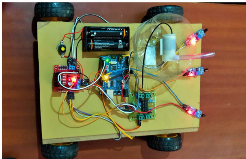
Fig-2: Fire Fighting Robot
