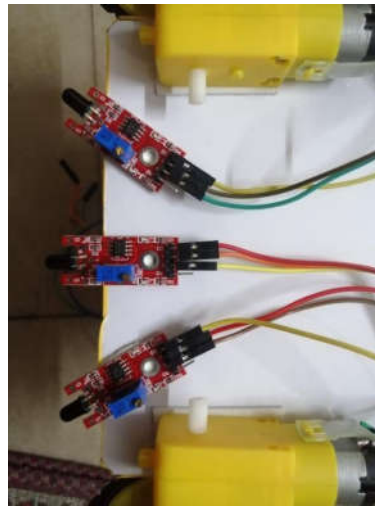
Fig-5:IR Flame Sensor
