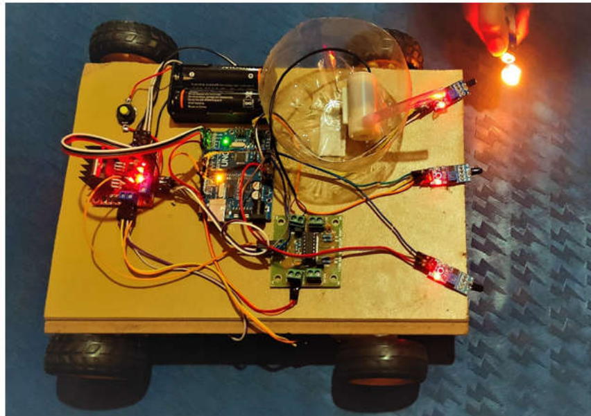
Fig-10:Fire Fighting Robot
